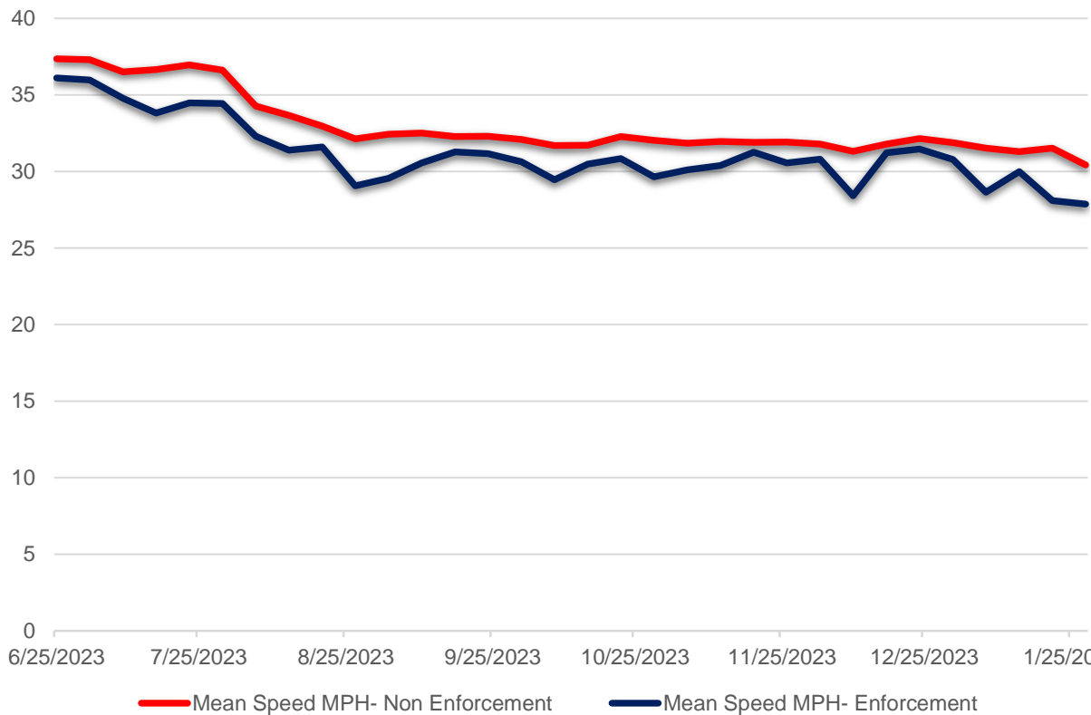
WESTBOUND - MEAN SPEED
