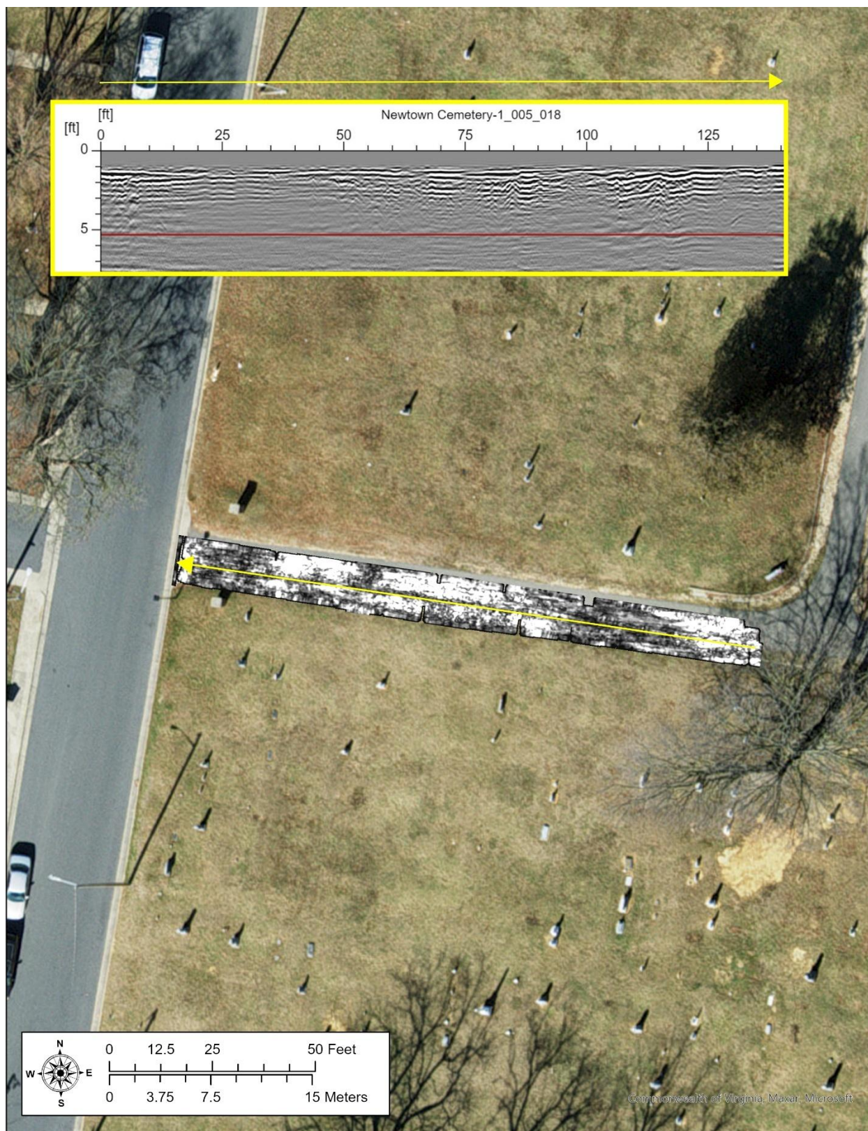
Figure 4.7. The Effinger Street MALA HDR survey and representative reflectance profile (inset).
