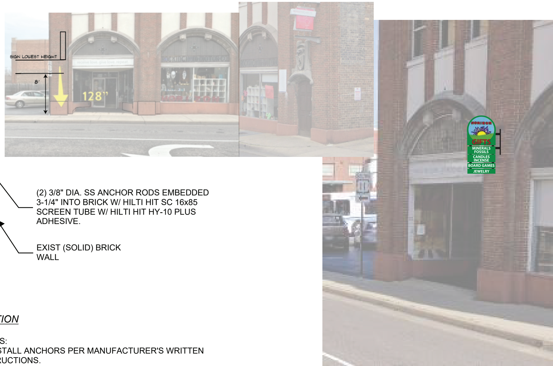
BUILDING ELEVATION/PERSPECTIVE NTS
